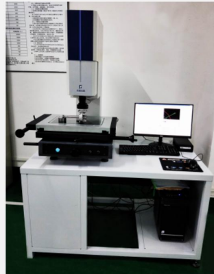
二维影像测量仪 Two-Dimensional Image Measuring Instrument
